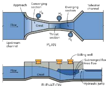
Figure 1.5.1: Diagram of a Parshall Flume by Inductiveload is in the public domain
