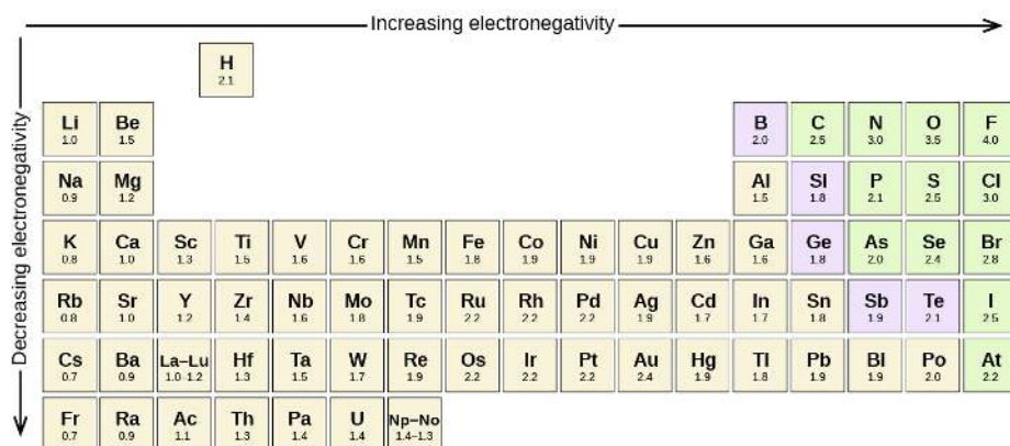
Figure 4.4.4 The electronegativity
