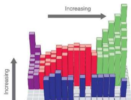
Electronegativity, \chi
