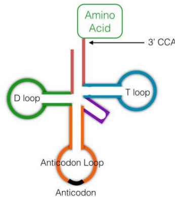
Figure 15.2.3: tRNA structure
