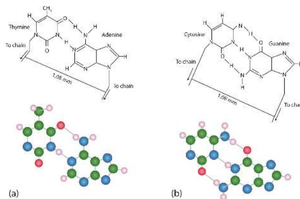
Figure 14.2.3 Complementary Base Pairing. Complementary bases engage in hydrogen bonding with one another: (a) thymine and adenine; (b) cytosine and guanine.
