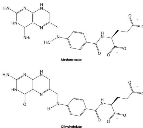
Figure 13.16.2 - Methotrexate and dihydrofolate. Image by Ben Carson
