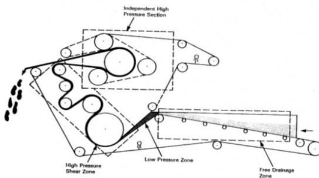
Figure 1.7.1: Filter Press - Image by the EPA is in the public domain
