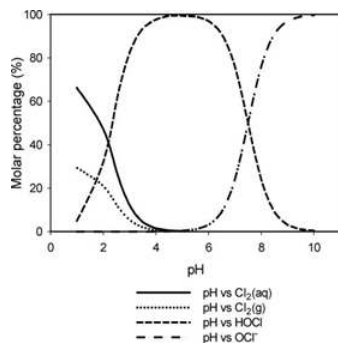
Figure 1.3.1: Title: Chlorination Curve - Description: pH values of chlorine on graph. Image by L. Wang, Ph.D., M. Bassiri, PhD, R. Najafi, Ph.D., K. Najafi, MD, J. Yang, BS, B. Khosrovi, Ph.D., W. Hwong, BS, E. Barati, BS, B. Belisle, Ph.D., C. Cereli, MS, and M.C. Robson, MD is licensed under CC BY
