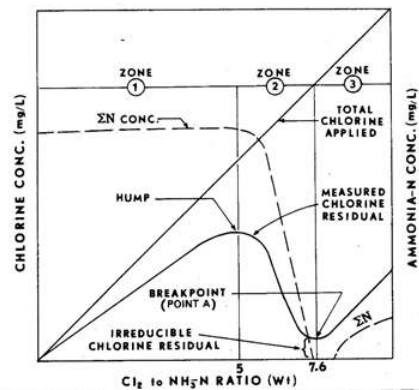
Figure 1.3.3: Title: Graph of breakpoint chlorination - Description: Breakpoint Chlorination Curve. © State of New South Wales NSW Ministry of Health. For current information go to www.health.nsw.gov.au . – Image licensed under CC BY 4.0
