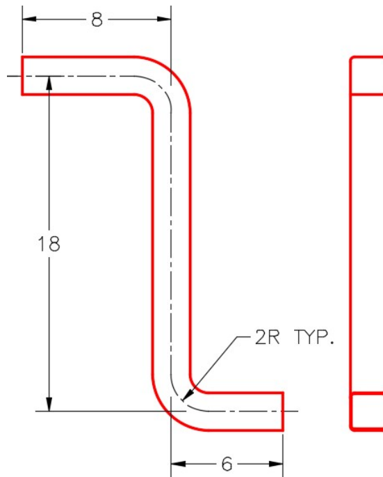
Figure Step 2A Dimensioned Multiview Drawing
