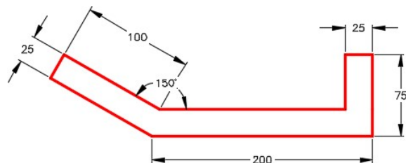
Figure Step 2C Front View – Base View
