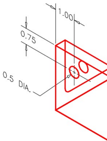
Figure Step 5A Hole Detail
