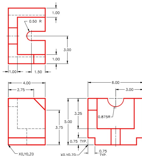
Figure Step 2A Dimensioned Multiview Drawing
