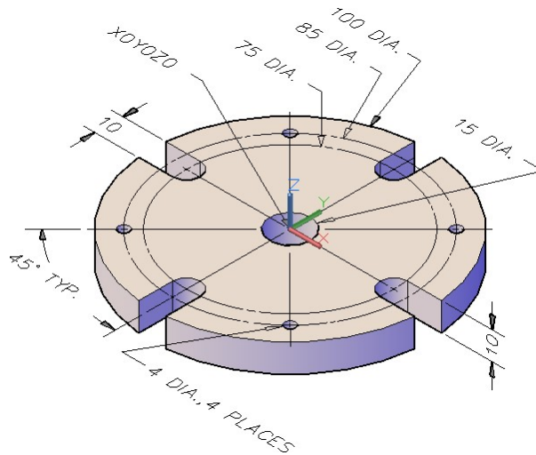
Figure Step 2 Dimensioned Solid Model
