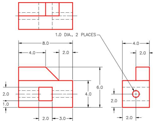
Figure Step 4A Dimensioned Multiview Drawing
