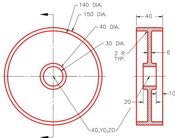
Figure Step 1A Dimensioned Multiview Drawing
