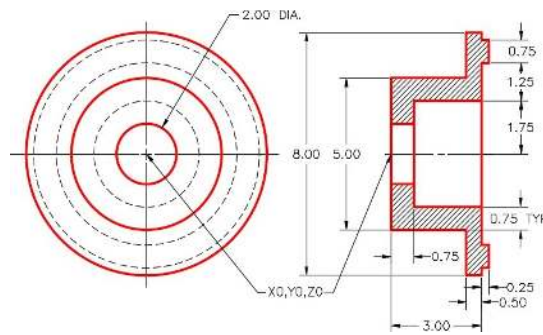
Figure Step 2 Dimensioned Multiview Drawing
