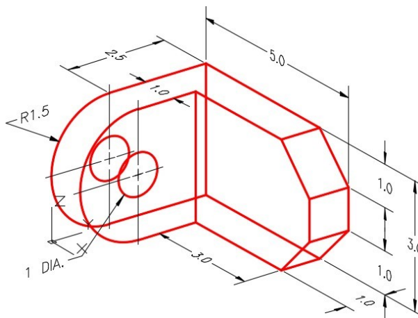
Figure Step 2A Dimension Wireframe Model
