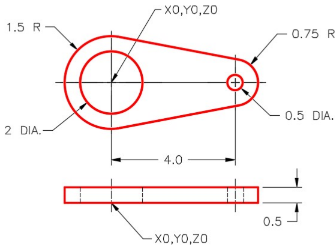
Figure Step 3A Dimensioned Multiview Drawing
