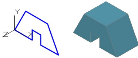
Figure 18-1 Extruding a Solid Model
