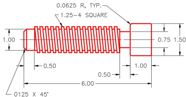
Figure Step 2A Dimensioned Multiview Drawing
