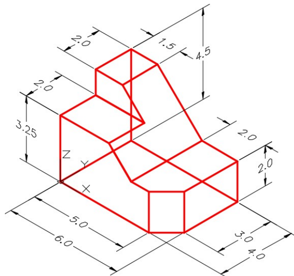
Figure Step 5A Dimensioned Wireframe Model
