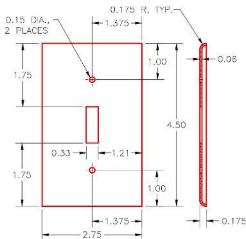
Figure Step 2A Dimensioned Multiview Drawing
