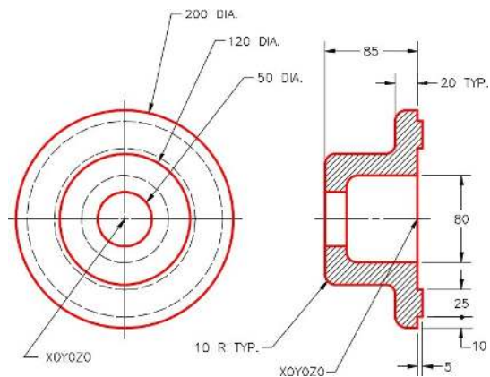
Figure Step 2A Dimensioned Multiview Drawing
