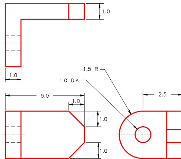
Figure Step 1 Dimensioned Multiview Drawing
