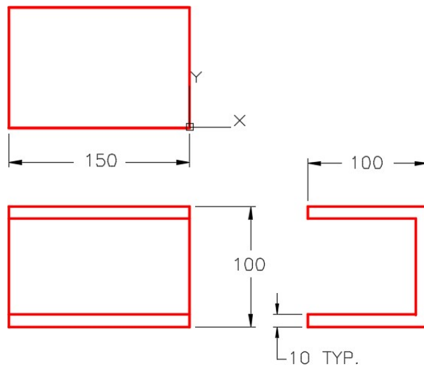
Figure Step 3B Dimensioned Multiview Drawing
