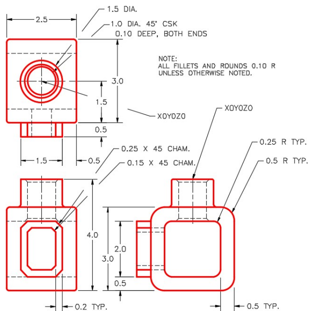
Figure Step 3B Dimensioned Multiview Drawing
