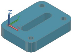
Figure Step 15 SE Isometric View
