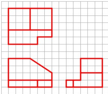
Figure Step 7A Multiview Drawing – Object 7-1
