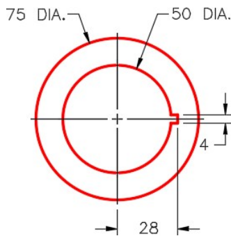
Figure Step 2E Detail of Keyway
