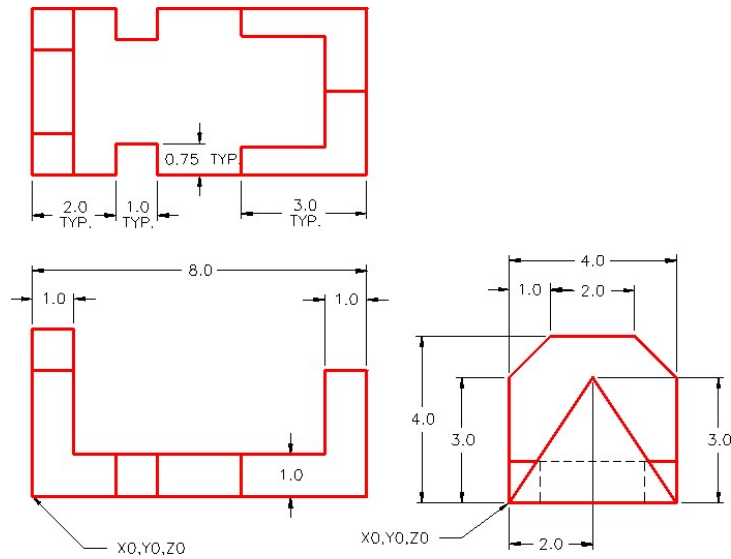
Figure Step 2A Dimensioned Multiview Drawing
