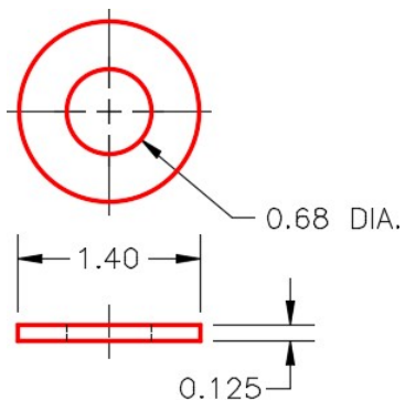
Figure Step 6A Dimensioned Drawing of Washer
