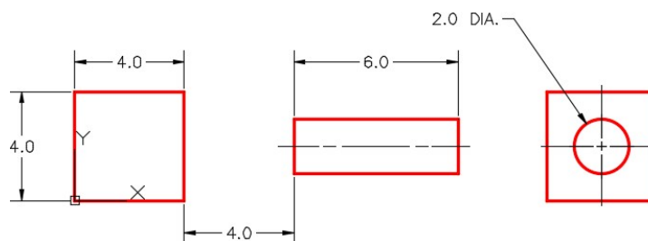
Figure Step 4A Dimensioned Multiview Drawing
