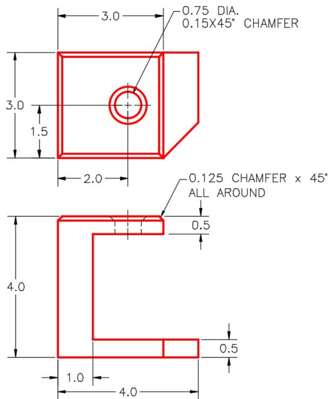
Figure Step 11A Dimensioned Multiview Of Model 2
