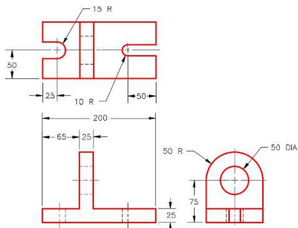
Figure Step 4B Dimensioned Multiview Drawing
