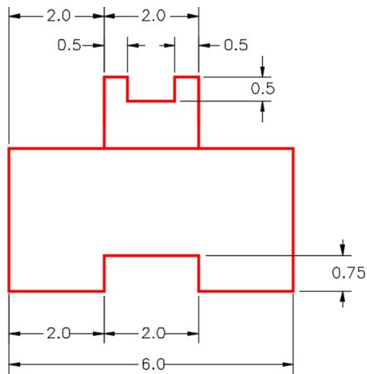
Figure Step 2F Detail of Rear View
