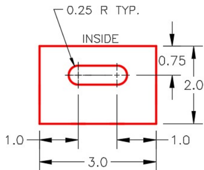
Figure Step 2D Bottom Detail TYP.
