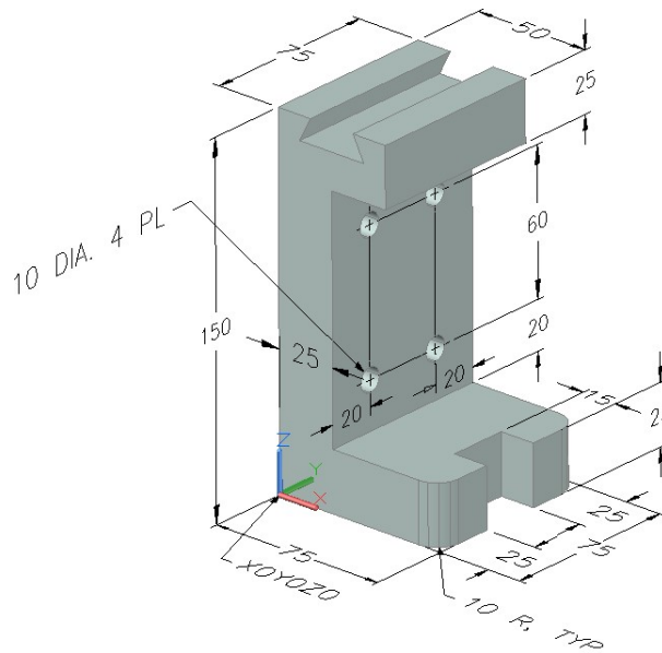
Figure Step 4A Dimensioned Solid Model
