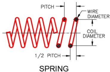
Figure 23-5 Threads and Spring Shape and Terminology
