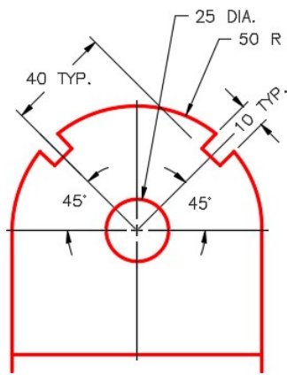
Figure Step 2D Detail of Inclined plane
