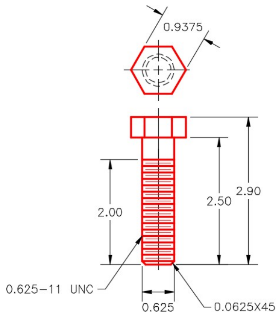
Figure Step 2A Dimensioned Multiview Drawing
