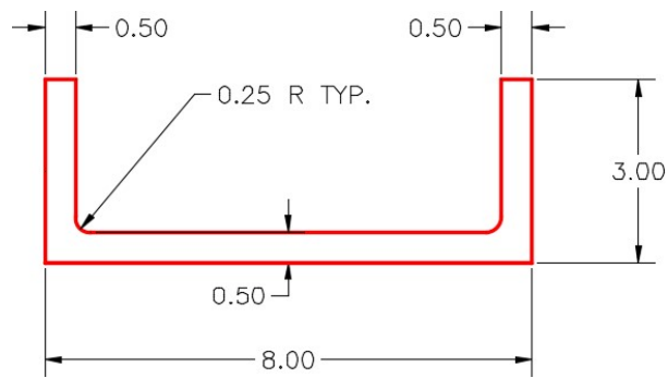
Figure Step 4A Right Side View
