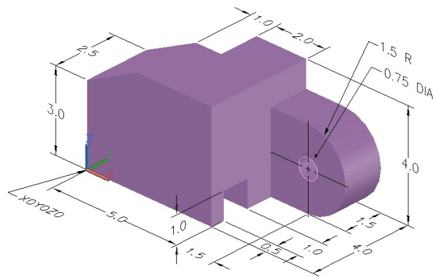
Figure Step 4A Dimensioned Solid Model
