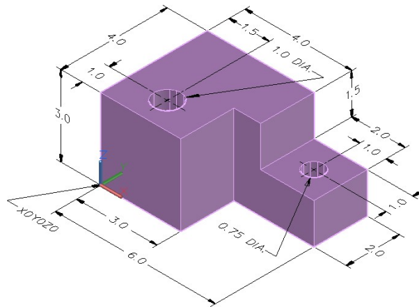
Figure Step 3A Dimensioned Solid Model
