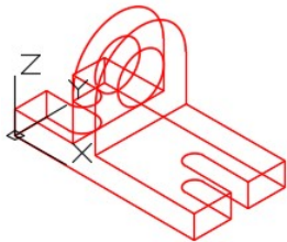
Figure Step 4A Wireframe Model
