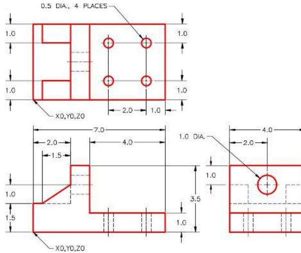
Figure Step 1A Dimensioned Multiview Drawing
