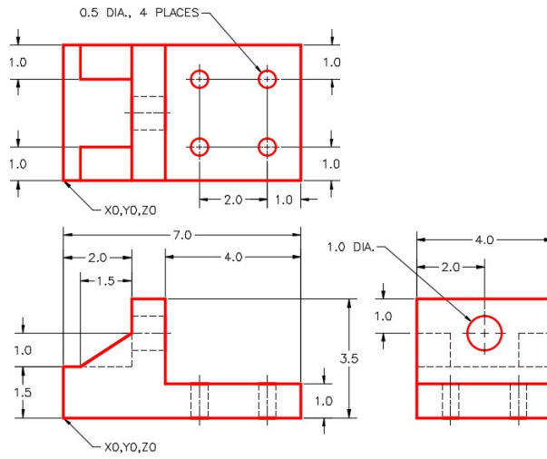
Figure Step 2A Dimensioned Multiview Drawing
