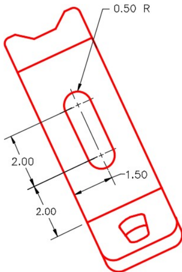
Figure Step 2B Auxiliary View
