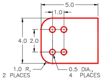
Figure Step 2F Detail of Bottom
