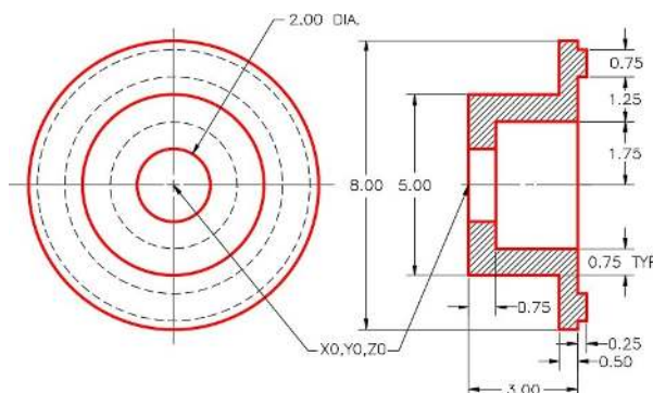
Figure Step 2 Dimensioned Multiview Drawing
