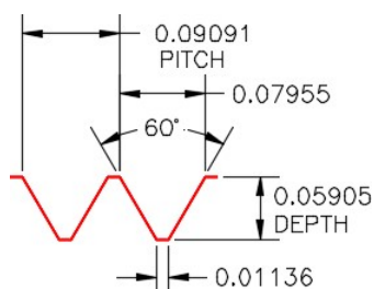
Figure Step 4B Dimensioned Thread Details
