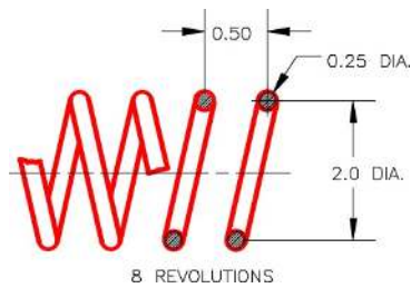
Figure Step 2A Dimensioned Drawing
