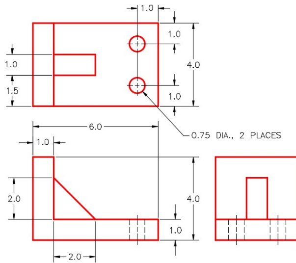
Figure Step 2B Dimensioned Multiview Drawing
