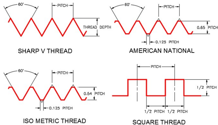
Figure 23-6 Four Common Thread Types
