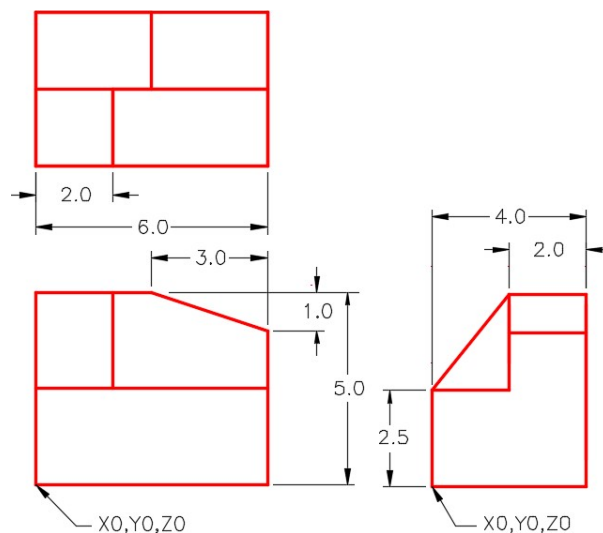
Figure Step 1A Dimensioned Multiview Drawing
