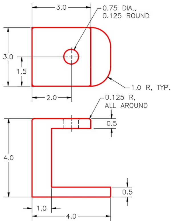
Figure Step 3A Dimensioned Multiview of Model 1
