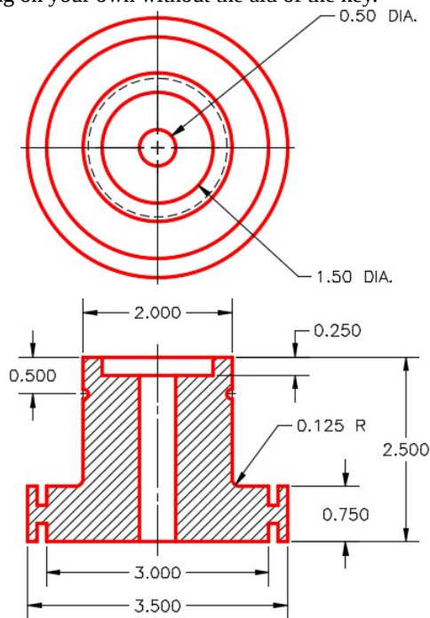
Figure Step 1A Dimensioned Multiview Drawing
