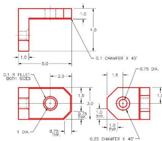
Figure Step 2A Dimensioned Multiview Drawing
