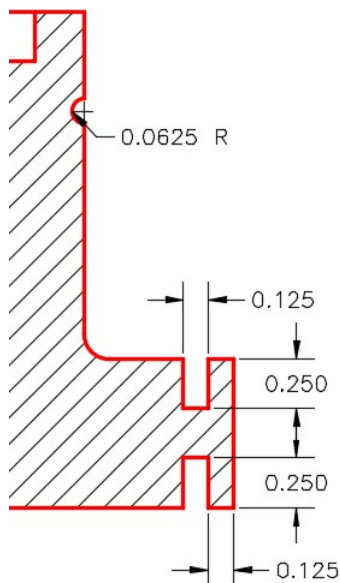
Figure Step 1B Dimensioned Detail
