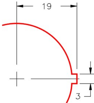
Figure Step 3C Key Detail
