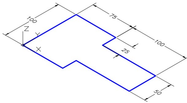
Figure Step 2 Dimensioned Drawing
