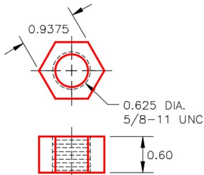
Figure Step 19A Dimensioned Multiview Drawing
