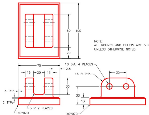
Figure Step 2A Dimensioned Multiview Drawing
