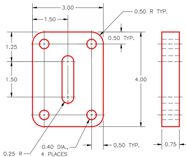
Figure Step 2 Dimensioned Multiview Drawing
