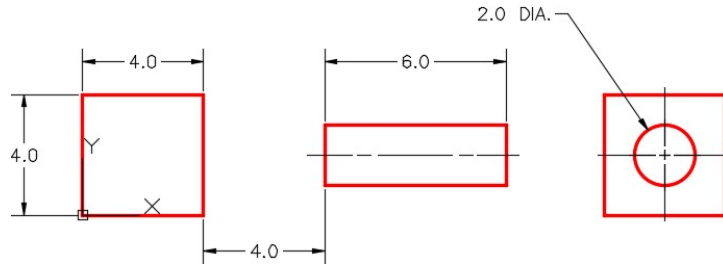
Figure Step 3A Dimensioned Multiview Drawing
