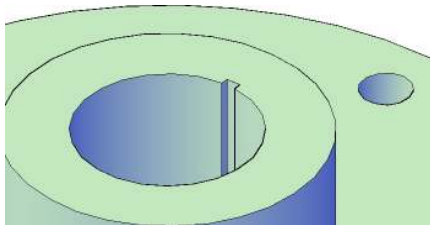
Figure Step 2B View of Keyway - Rotated
