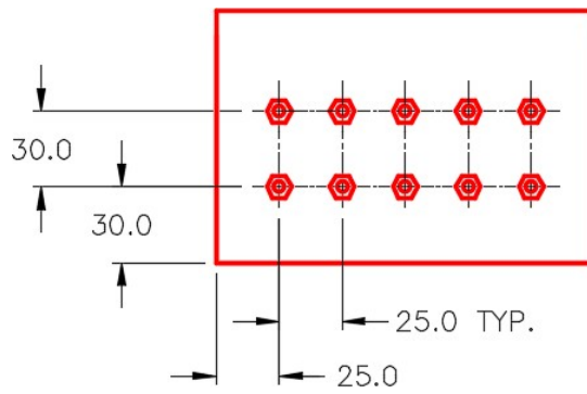
Figure Step 5A Bolt Pattern – Bottom View
