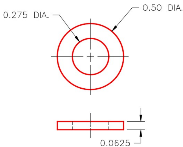
Figure Step 3B Dimensioned Multiview Drawing of the Washer
