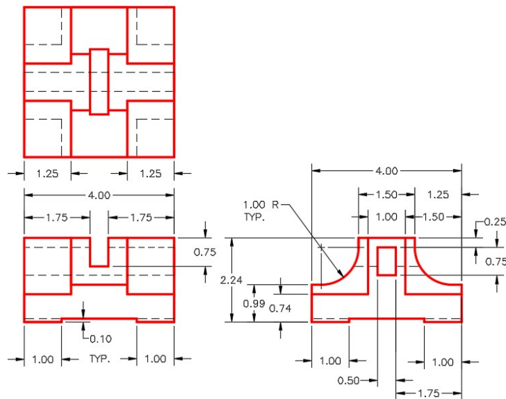
Figure Step 1B Dimensioned Multiview Drawing
