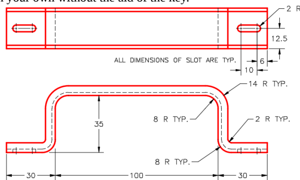
Figure Step 1A Dimensioned Multiview Drawing
