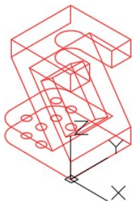
Figure Step 2B Completed Wireframe Model
