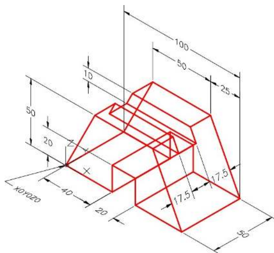
Figure Step 1A Dimensioned Wireframe Model
