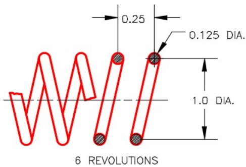
Figure Step 7A Dimensioned Drawing of Spring
