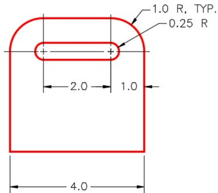
Figure Step 2E Detail of Inclined View
