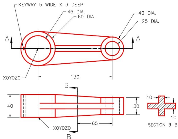
Figure Step 2B Dimensioned Multiview Drawing
