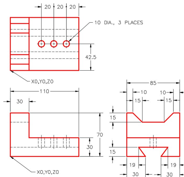
Figure Step 1A Dimensioned Multiview Drawing
