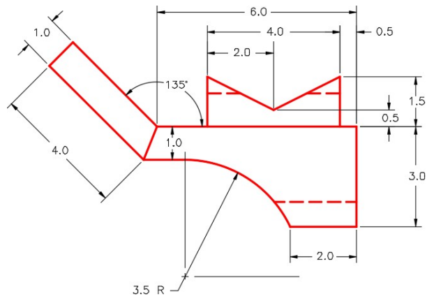
Figure Step 2D Right Side View
