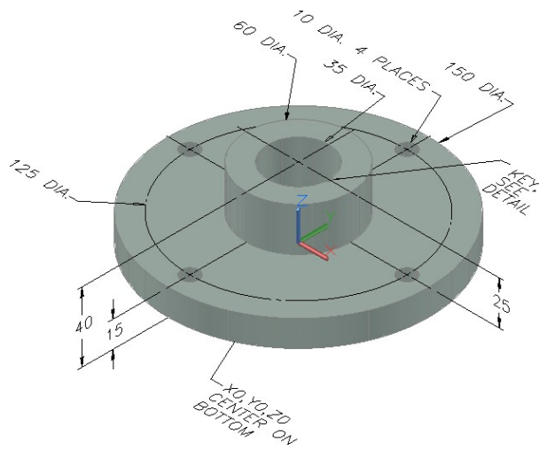
Figure Step 3A Dimensioned Solid Model
