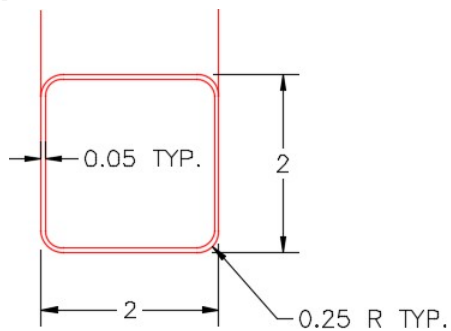
Figure Step 2C Dimensioned Detail of Opening
