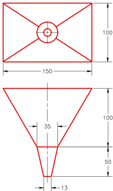
Figure Step 1 Dimensioned Multiview Drawing
