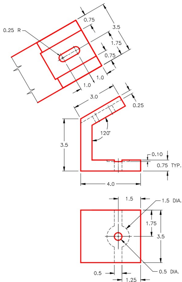
Figure Step 3C Dimensioned Multiview Drawing
