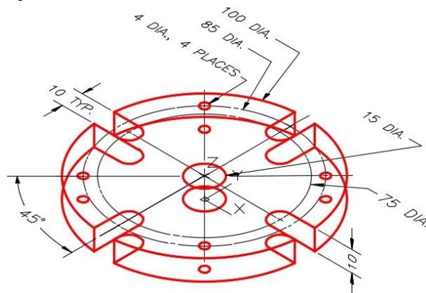
Figure Step 1B Dimensioned Wireframe Model
