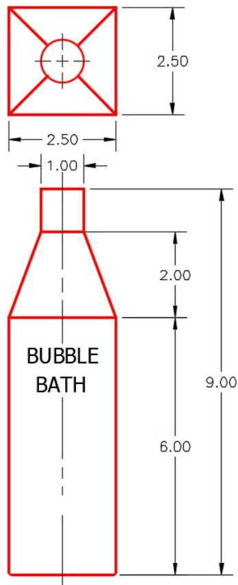
Figure Step 1 Dimensioned Multiview Drawing
