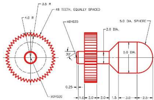
Figure Step 2A Dimensioned Multiview Drawing
